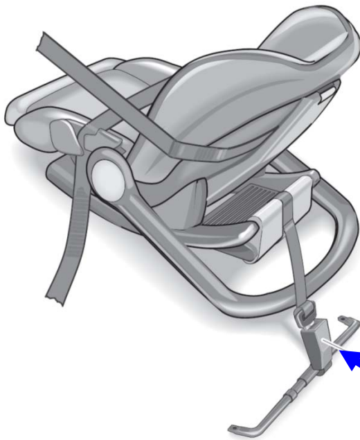
Traverse Airbag Deactivation (996.803.083.02) under passenger seat in 9X6 vehicles
