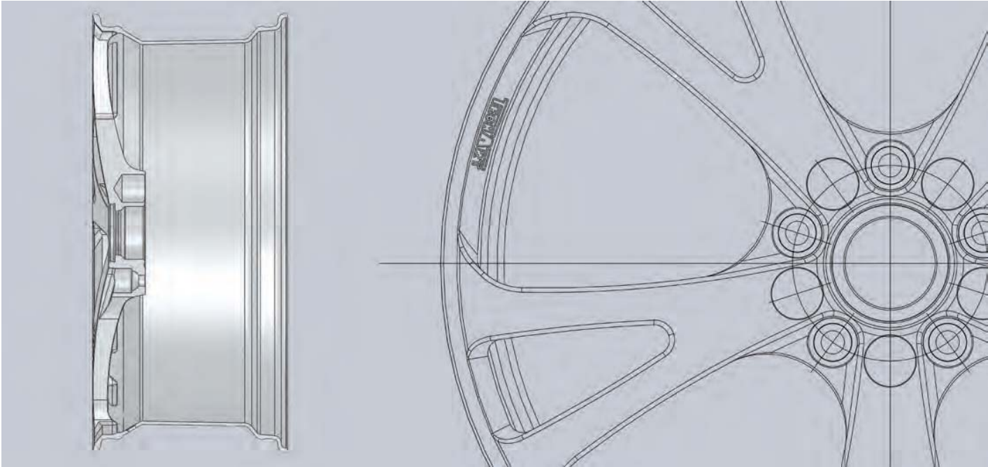
Einzigartiges Design, modernste Schmiedetechnologie, optimale Reduzierung ungefederter Massen. Das TECHART Formula III Schmiederad mit fünf dynamischen Doppelspeichen. Unique design, state of the art forging technology, optimized reduction of the unsprung mass. The TECHART Formula III forged wheel with five dynamically shaped twin-spokes.
